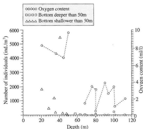
Fig. 4. Biomass distribution in the changing depth and dissolved oxygen content of the sampling stations
