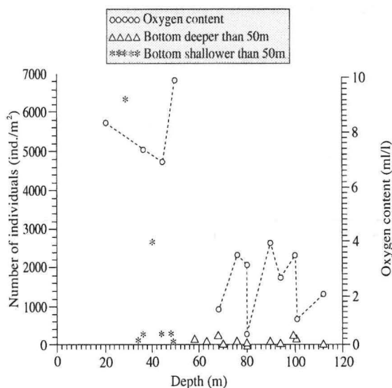
Fig. 2. Changes in individual number of macro-benthic crustacean with the depth and dissolved oxygen content
