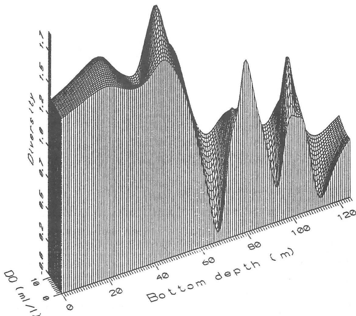
Fig. 5. Three-dimensional demonstration of relationship between Shannon Weaver's diversity, depth and dissolved oxygen content along the coast of the Southern Black Sea
