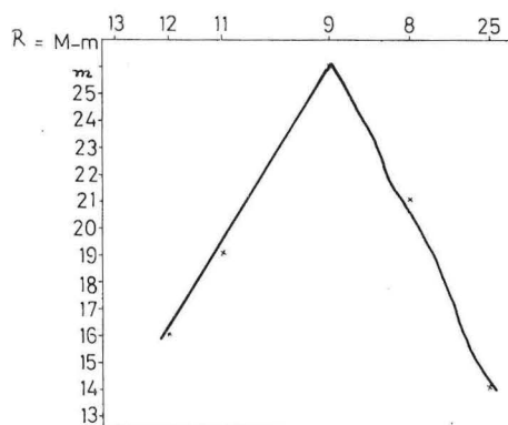
Fig. 62. Long term variations of sea transparency measured by Secchi disc at Split—Gargano cross-section (Stations 13—25) presented by ranges (R = maximum — minimum).
