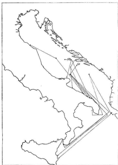
Fig. 54. Drift bottle movements for September.
