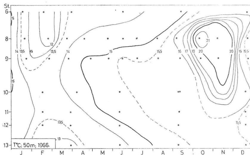
Fig. 11. Temperature distribution at 50 m depth at Split—Gargano cross-section in 1966.
