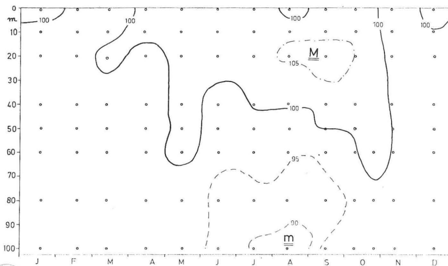
Fig. 65. Normal distribution of O_2 % at Station 9 (Stončica). Means were computed from the data for eight years.
