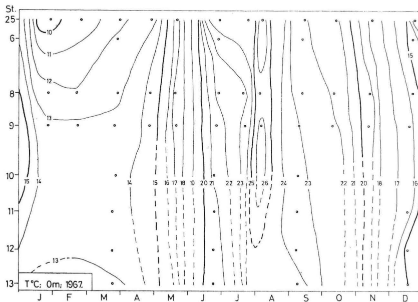
Fig. 6. Distribution of sea surface temperatures at Split—Gargano cross-section in 1967.
