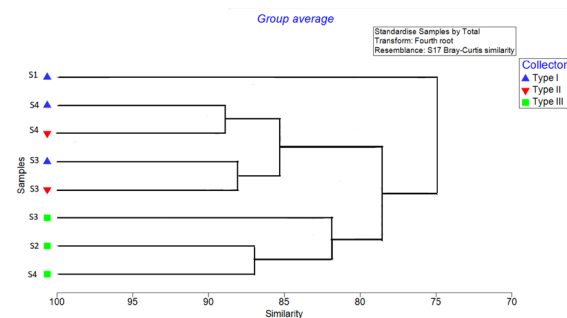
Fig. 4. Similarity of sites by shellfish species on collectors (Bray-Curtis method)
