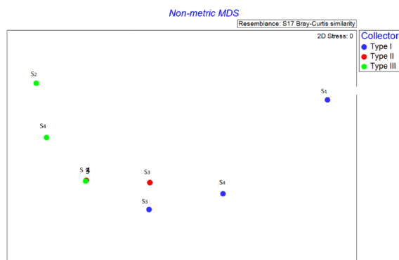
Fig. 3. MDS grouping of sites by shellfish species on collectors
