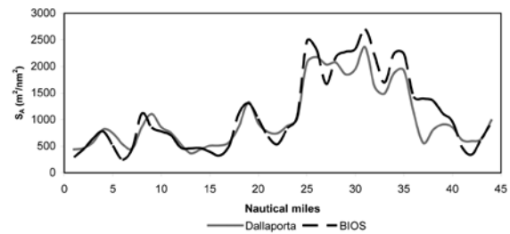
Fig. 3. Comparison of S_A -values measured by the two research vessels during the first mini-survey (night) in the Neretva Channel
