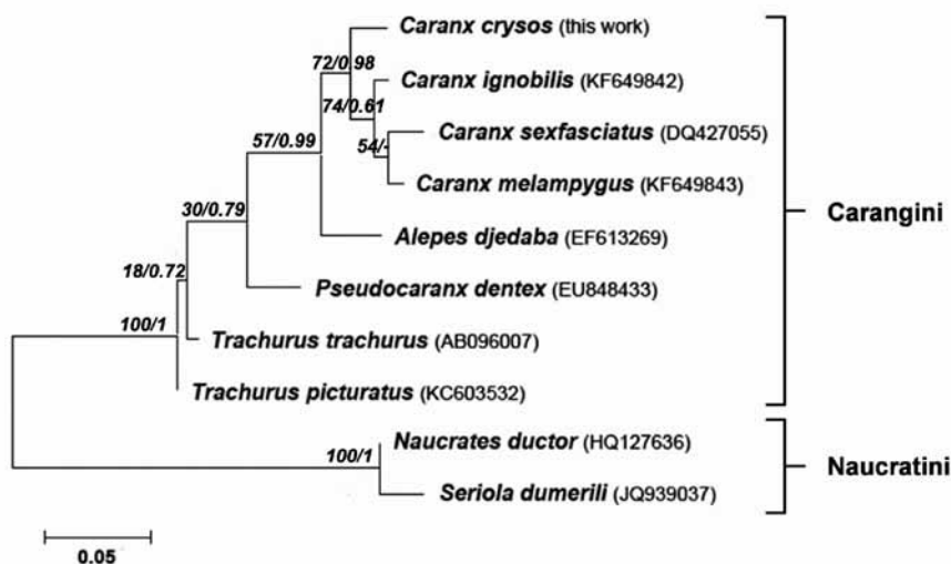
Fig. 4. The ML/Bayesian phylogenetic tree of 16S rDNA sequences from Caranx crysos and related carangids. The accession numbers of the sequences from carangid representatives retrieved from the GenBank database are indicated in the parenthesis. Numbers on branches indicate ML bootstrap support / Bayesian posterior probabilities
