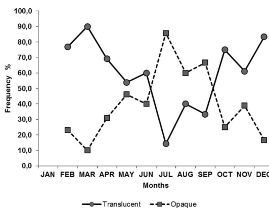
Fig. 4. Categorization of the otolith edges by month for the Atlantic bonito sampled in the Eastern Mediterranean Sea. Lines correspond to the percentages of the opaque and translucent bands observed at the margin of otolith sections
