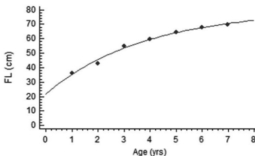
Fig. 5. Von Bertalanffy growth curve for the Atlantic bonito sampled in the eastern Mediterranean Sea. Black dots indicate mean observed lengths at age estimated from sectioned otolith reading
