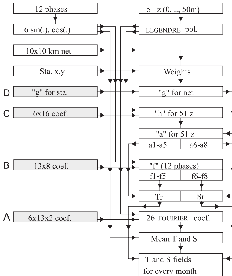
Fig. 3. Reconstruction of temperature (T) and salinity (S) fields from four tables of coefficients. Arrows indicate direction of data flow
