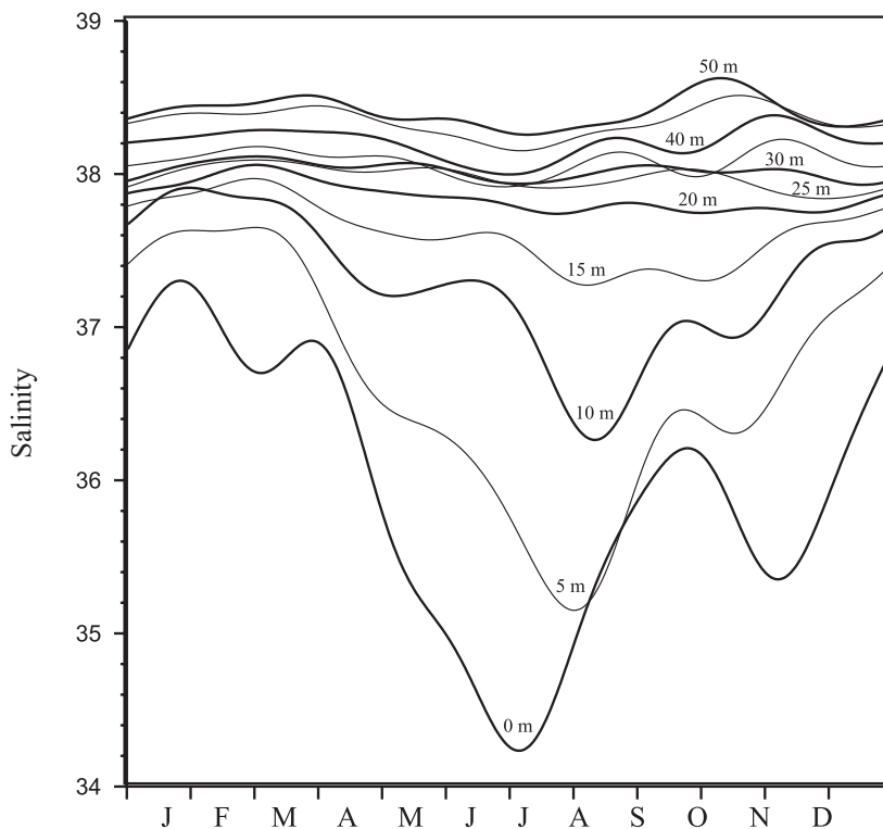
Fig. 5. Annual mean salinity cycle in the northern Adriatic
