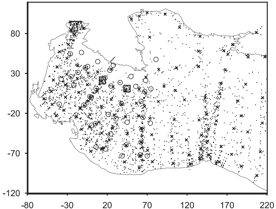
Fig. 1. Northern Adriatic area included in the study. The origin is at 45^\circ\text{N} , 13^\circ\text{E} . The x coordinate is in the SE direction and the y coordinate in the NE direction, expressed in km. Dots – MEDATLAS data, crosses – fictitious stations, circles – CMR stations. Circles inside squares – stations SJ107 (left) and SJ209 (right)
