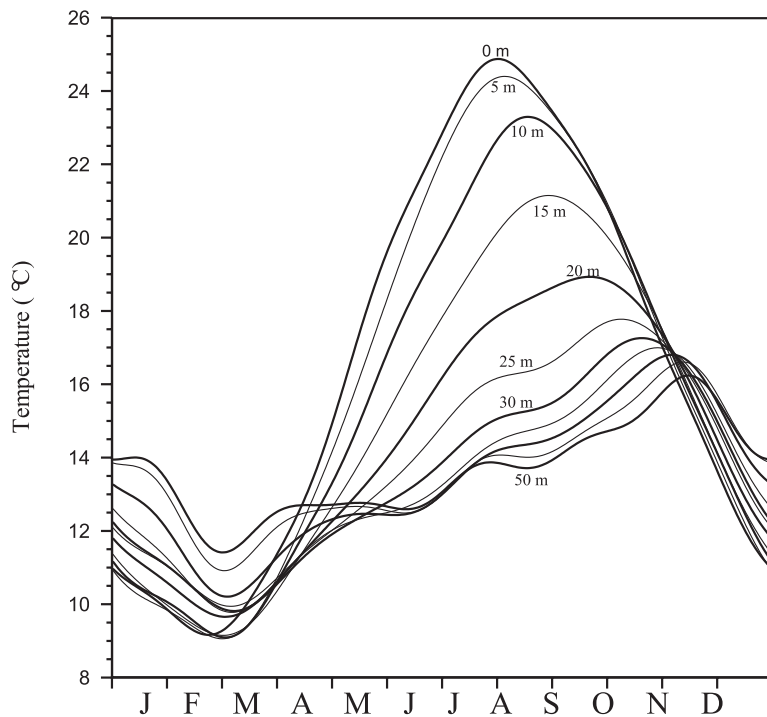
Fig. 4. Annual mean temperature cycle in the northern Adriatic
