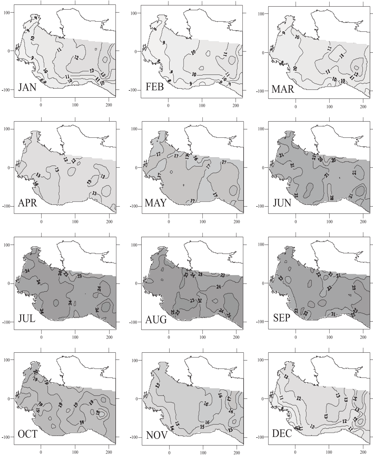
Fig. 6. Climatology of sea surface temperature in the northern Adriatic
