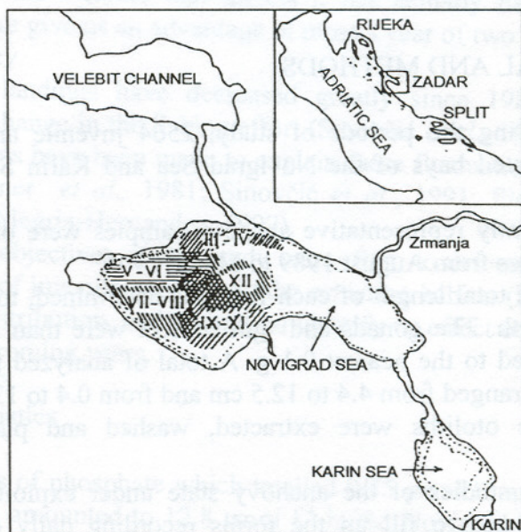
Fig. 1. Map showing the investigation area as well as the spatial and temporal distribution of juvenile anchovy in the Novigrad Sea during 1990
